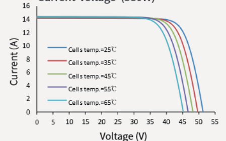
Current-Voltage (580W)
